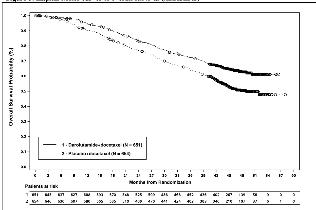
Figure 3: Kaplan-Meier curves of overall survival (ARASENS) a
